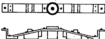
D&RGW Bolsters for Short Caboose or Reefer #64 in brass, #1064
