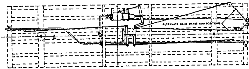
NY Air Brake Set, Type K, 8" x 8" #4064
