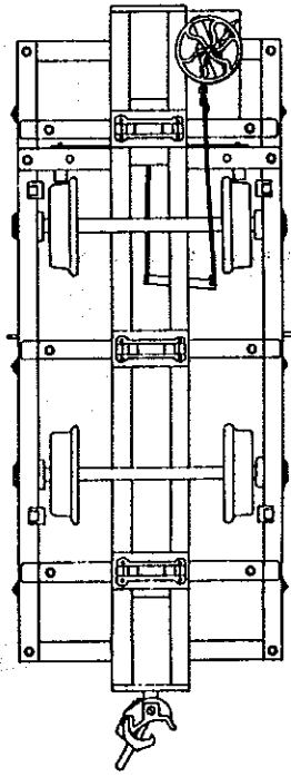
FIGURE 3: Top View--Frame
