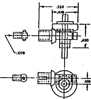
2:1 Ratio Gears, Cross Box .078" Bore U-Joint 1/8" Axle #7086 3mm Axle #7085
