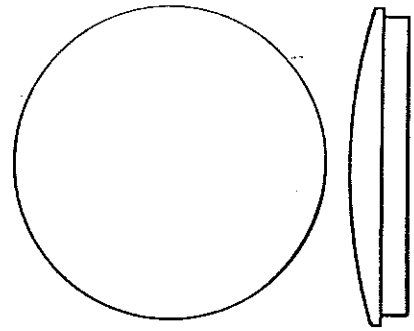
D&RGW Tank Car Ends 77" Diameter #12
