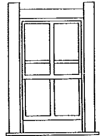
Double Hung Window 4 Pane, 31" x 56" Operating Sash Sargents Station #3711
