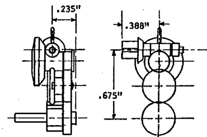
4:1 Ratio Gear Tower .078" Bore U-Joint 3/32" Axle Bore (wheels not included) #7013
