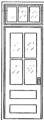
Factory Front Door 39" x 92" for Masonry Building #3612
