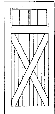
Freight Doors--Double 4' x 9' with window #3611
