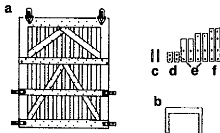
Stock Car Door, End Detail D&RGW #4005
