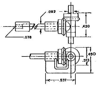
1:1 Gears--In line Mounting Bracket .089" Coupling 3/32" Axle Material (will clear wheels as small as .320" Diameter, 24" Gauge) #7037
