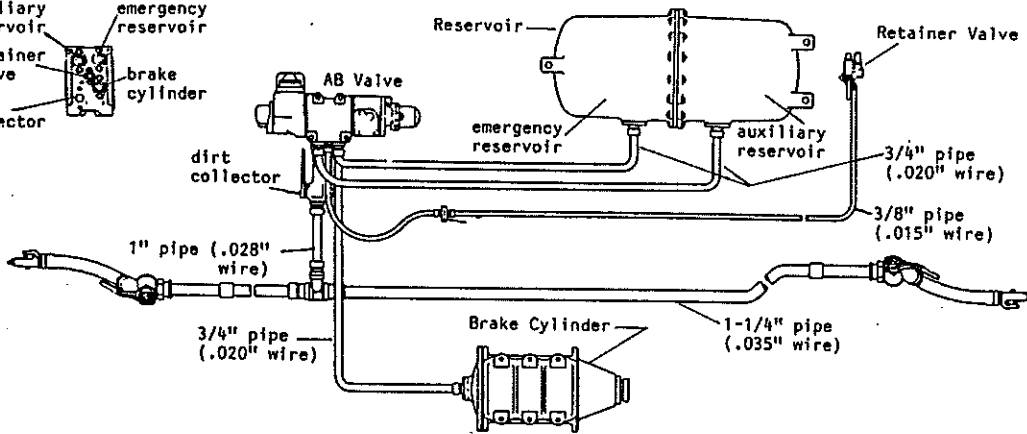
Piping Diagram
