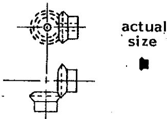
Bevel Gear 8 Tooth 1/8" OD, 1/32" Bore #7007
