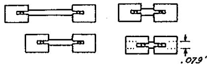
Universal Joints 0.6" to 1.0" overall length to fit .079" (2mm) Shafts #7011
