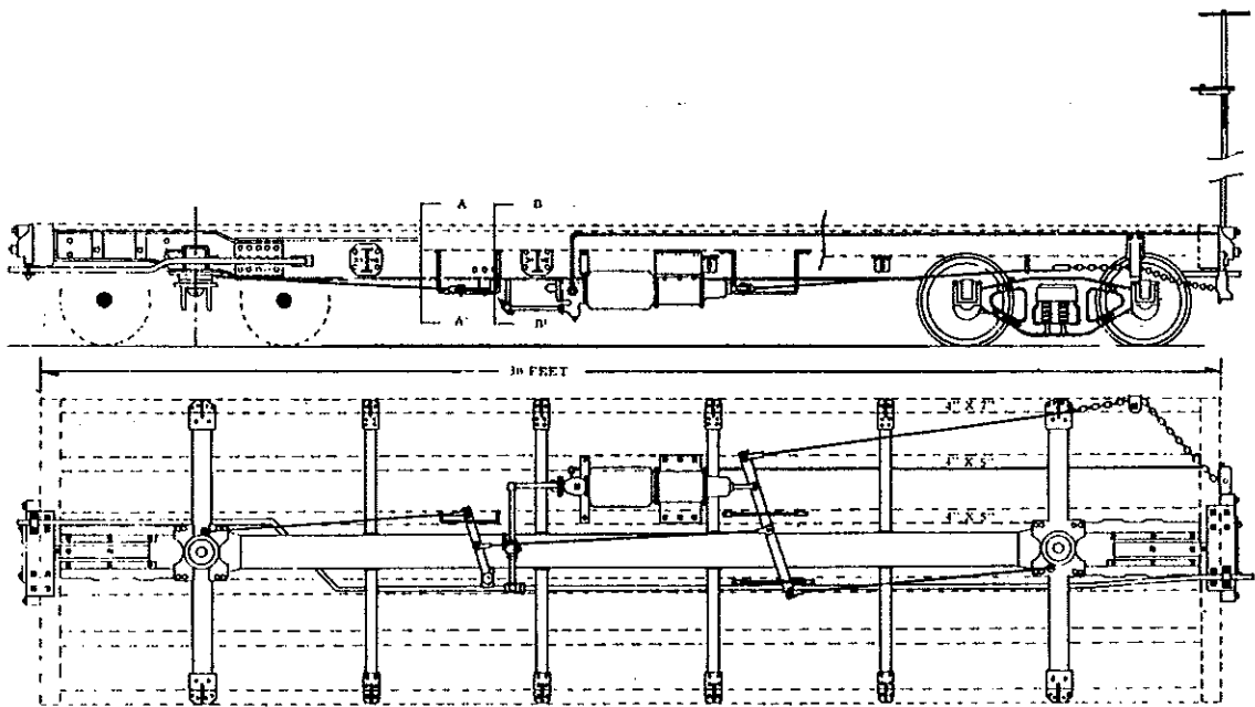
Bettendorf Steel Underframe Kit #3058 Contains hardware parts to construct a complete Bettendorf Underframe, including brakes, trucks, and couplers for a C&S Steel Underframe House Car. Some modification is required to construct a gondola.
