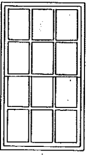
Double Hung Factory Window for Masonry Building 12 Pane, fits opening 42" x 72" #3718
