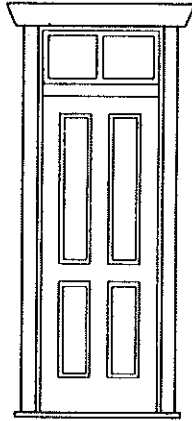
30" Station or House Door Separate Frame, Transom #3603
