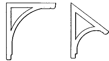
Eave and Gable Brackets #3516
