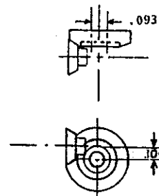
2:1 Skew Bevel Gears .062" and .093" Bore .100" Offset #7012
