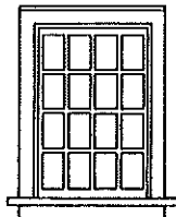
Double Hung Window 36" x 56", 16 Pane #4026
