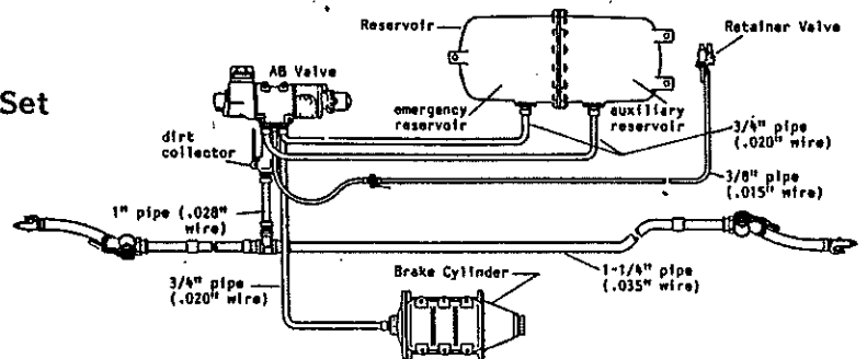
Piping Diagram
