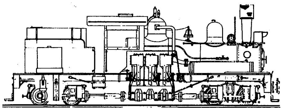
Micro-Mo Motor and Gearing for Kemtron Shay #7051
