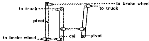
D&RGW Caboose Brake Levers #84
