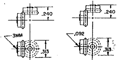
1:1 Bevel Gears, in line 15 Tooth .3mm Bore, 48 DP #7034 with 3/32" Bore, #7035
