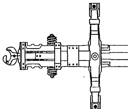
D&RGW High-side Gon Economy Draft Gear, Bolster Set #120
