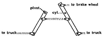
D&RGW Gon Brake Levers, Clevises #47
