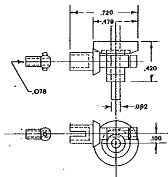
2:1 Ratio Gears, Cross Box .078" Bore U-Joint 3/32" Axle Material (Wheels not included) #7036
