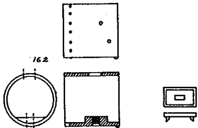
Top mounting Headlight Bracket Extended Smokebox Can be used for 8 Ton Porter #162
