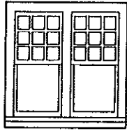
RGS Style Depot Windows 10 Pane, 32" x 54" 20 Pane, 58" x 60" #4041
