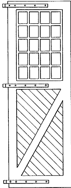
Engine House Door 5'2" x 15'3" with Hinges #3609
