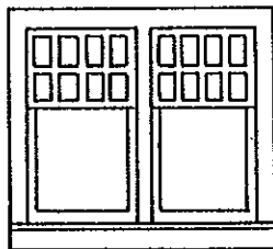
RGS Style Depot Windows 32" x 52", 9 pane 72" x 82", 18 pane 3742:
