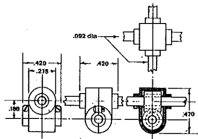
1:1 Helical Gears .1875" Offset Delrin Gearbox .078" Coupling #7038
