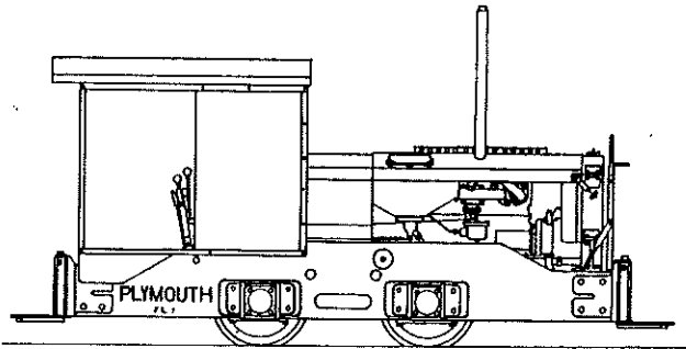
Plymouth FL-1 Six Ton Locomotive Unpowered On2 Kit #3019
