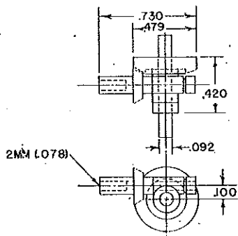
2:1 Ratio Gears, Cross Box, .078 Coupling 3/32" Axle Material Without Wheels, #7030 With 2 24" Spoked Wheels, #7031
