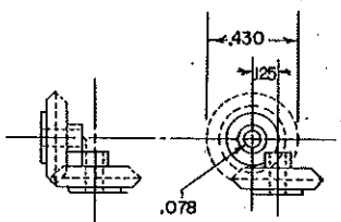
1:1 Skew Bevel Gears .078" Bore, .125" Offset #7077
