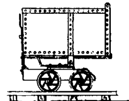
Rotary Mine Car 18" Gauge #3024 in brass, #2124
