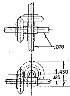
1:1 Skew Bevel Gears 1/8" Offset .078" Bore Cross Box with Axle Material #7040
