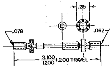
Universal Joint Set for Climax #7039
