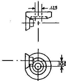
2:1 Skew Bevel Gears .062" and .125" Bore .100" Offset #7078
